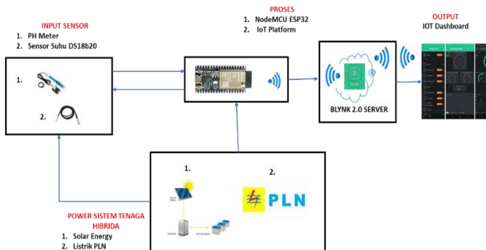
Gambar 6. Proses kerja alat sistem monitoring berbasis IoT
